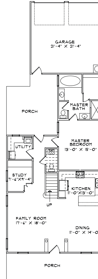
FIRST FLOOR PLAN 1294 SQ.FT.
