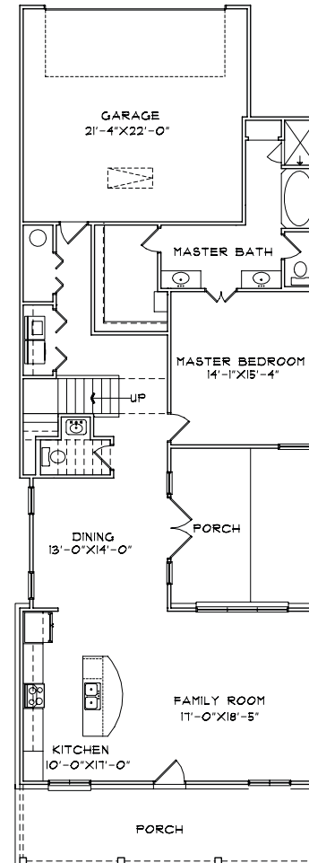
FIRST FLOOR PLAN 1449 SQ.FT.
